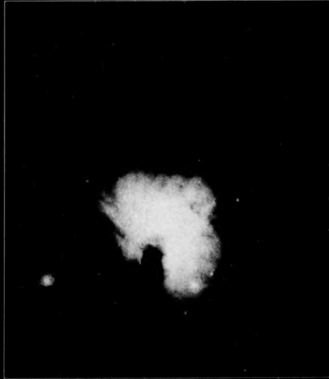
ORION NEBULA
