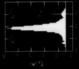
ORION NEBULA INFRARED SPECTRUM (CARBON ISOTOPES)
